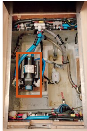
ON/OFF switch on fresh water pump located in starboard companionway.
