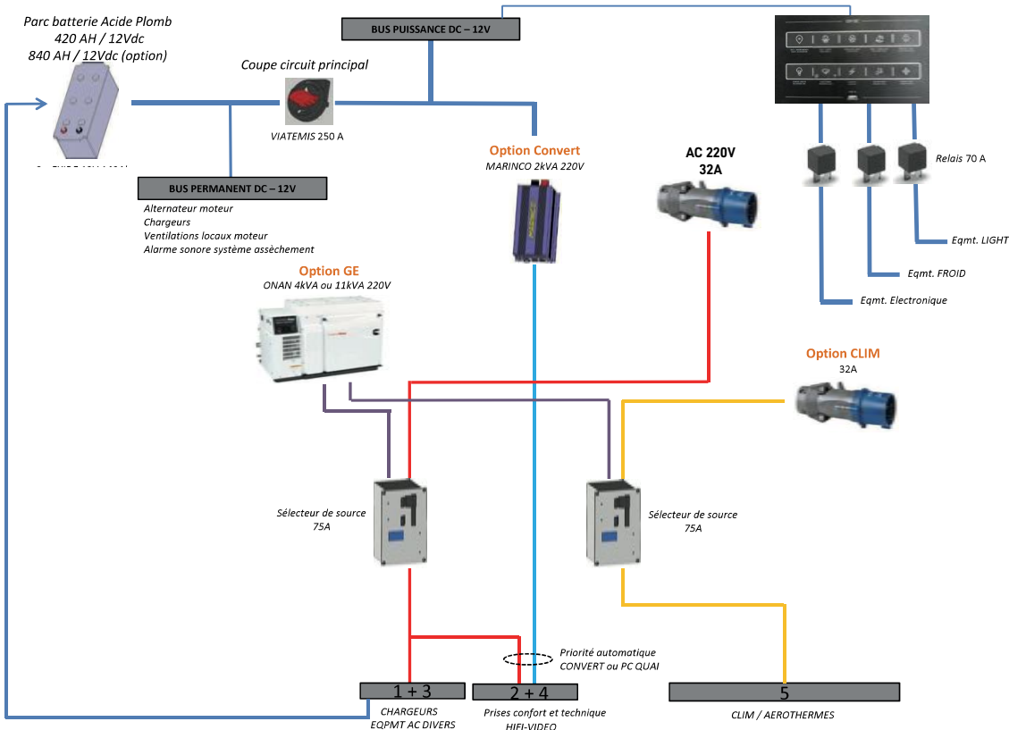
230V/50Hz Electrical circuit [complete circuit= standard + option]
