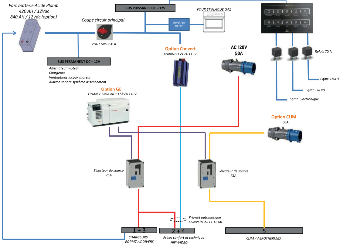
120V/60Hz Electrical circuit [complete circuit= standard + option]
