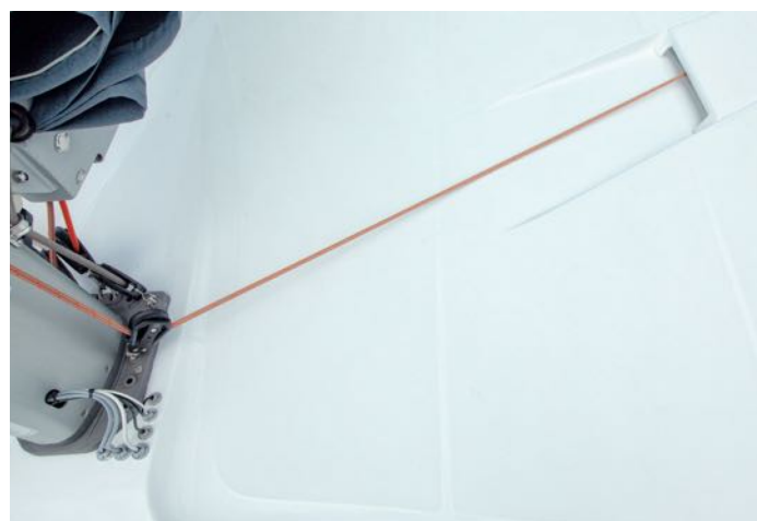
Roof foot block Rutgerson® - [Port]
