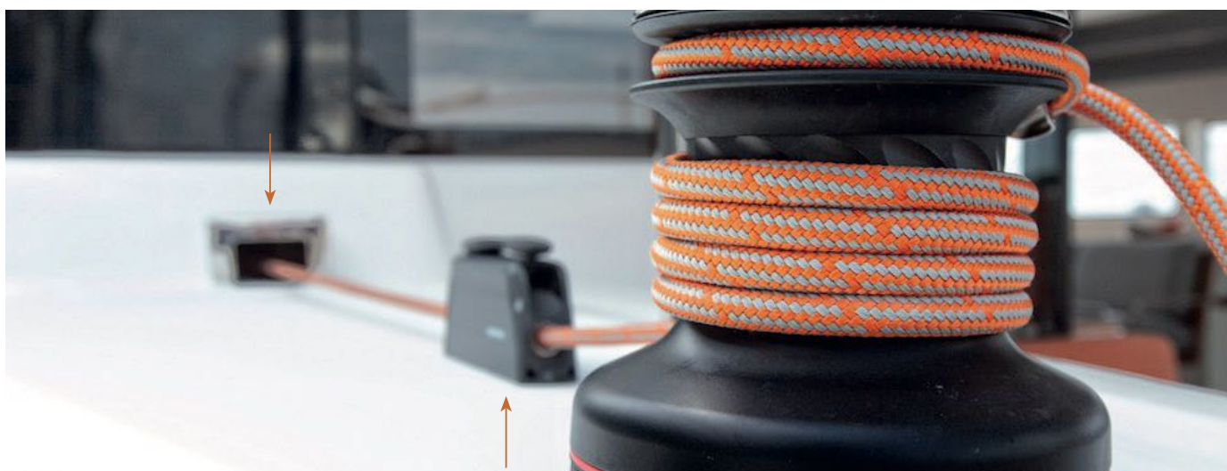
Deck foot block Rutgerson® - [Port] Jammer Spinlock® - [Port]
