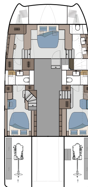
STANDARD 3 CABIN
