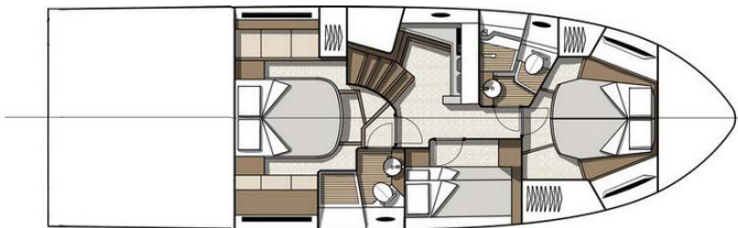
3-cabin layout
