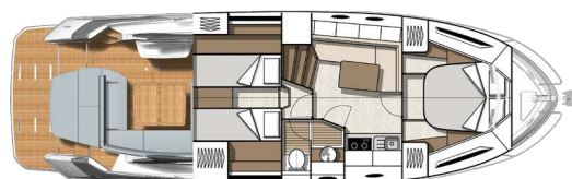
Lower deck
