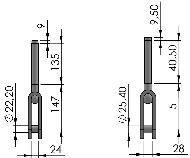
Toogle 7/8"
