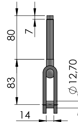
1/2" Toogle
