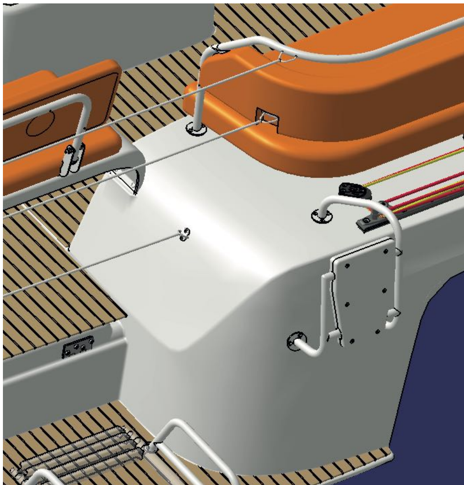
Stainless steel fixed bracket for dinghy outboard engine. Location: to port, on the aft beam.
