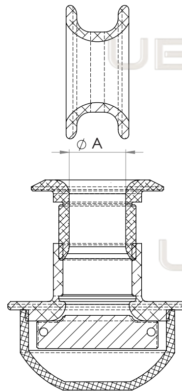
SECTION
