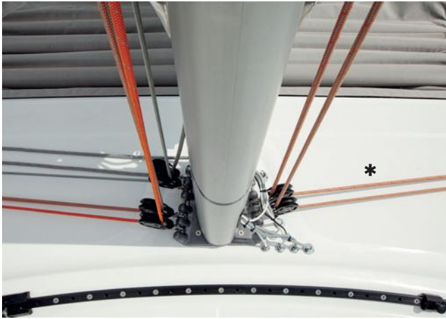
Mast foot block Code 0 halyard
