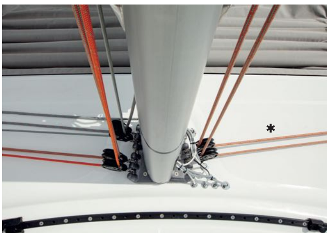
Mast foot block Code 0 halyard
